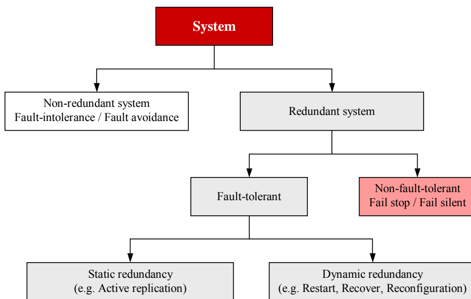
Figure 3. System redundancy due to Askerdal et al. (2000).
