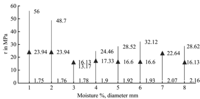
Figure 8 Moisture, diameter of specimens vs shear stress for Kora variety at bottom position
