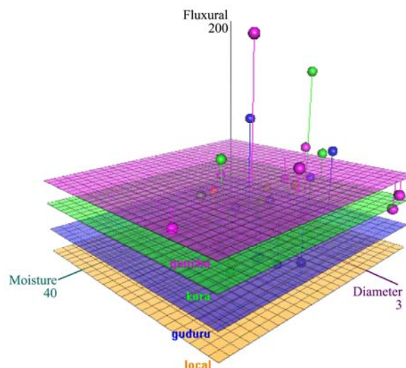
Figure 13 The effect of moisture and diameter of each varieties on flexural rigidity at bottom position / 3-D plot/
