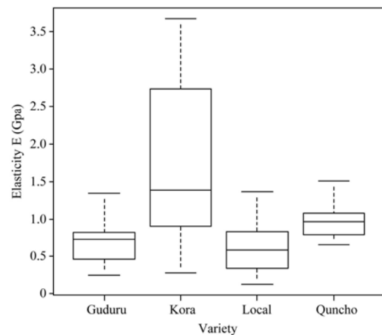
Figure 10 Comparison of Tef varieties on their maximum, minimum and mean value modulus of elasticity at bottom position
