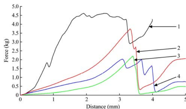
Figure 6 A typical shear (cutting) curve (graph) on the shearing strength test by texture analyzer 1 st kora variety (black), 2 nd local variety (red), 3 rd quncho variety (green), 4 th guduru variety (blue)
