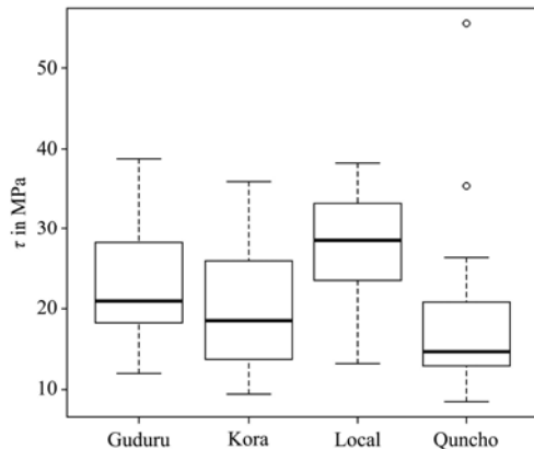
Figure 7 Comparison of Tef varieties on their max.,min. and mean value of shear stress at bottom position (segments)
