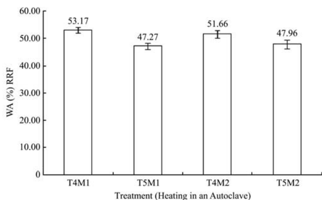
Figure 4 WA (%) of RRF heated in an autoclave
