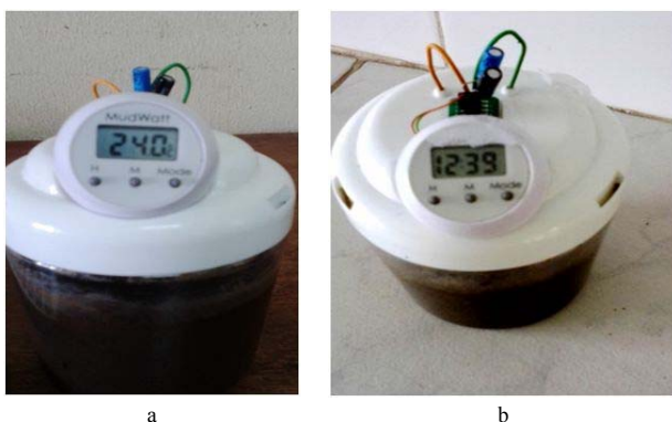
Plate 3 MFC urine powering (a) electronic clock (b) digital thermometer
