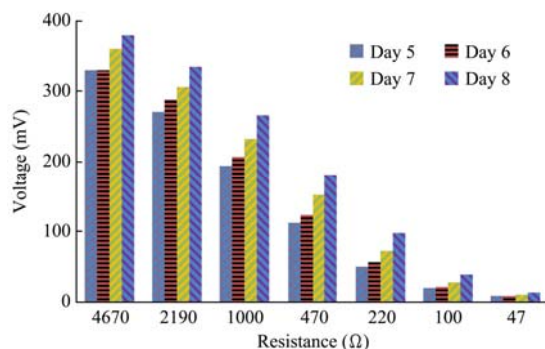
Figure 3 Measured voltages across external loads prior to urine addition (Days 5-8)
