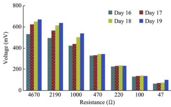
Figure 5 Voltage drop across external loads prior to urine addition (Days 13-16)
