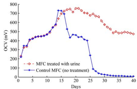
Figure 9 Daily OCV of urine treated MFC and the control MFC
