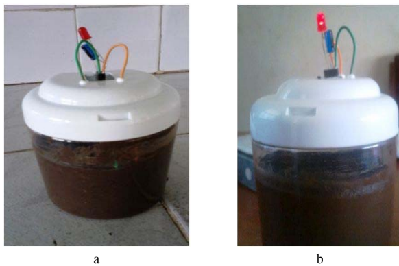
Plate 2 MSCMFC (a) before powering a LED (b) powering the LED
