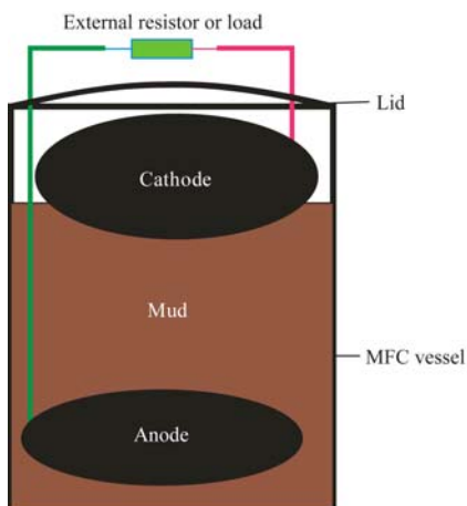
Figure 1 Schematic diagram of the MFC set-up (Source: Simeon et al., 2016a)
