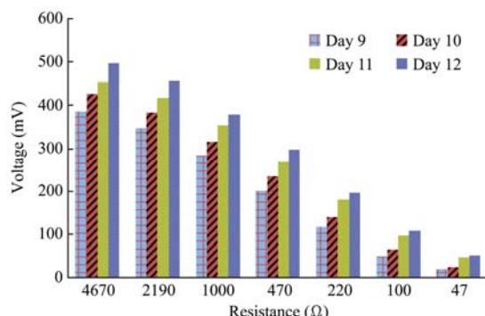
Figure 4 Voltage drop across external loads prior to urine addition (Days 9-12)
