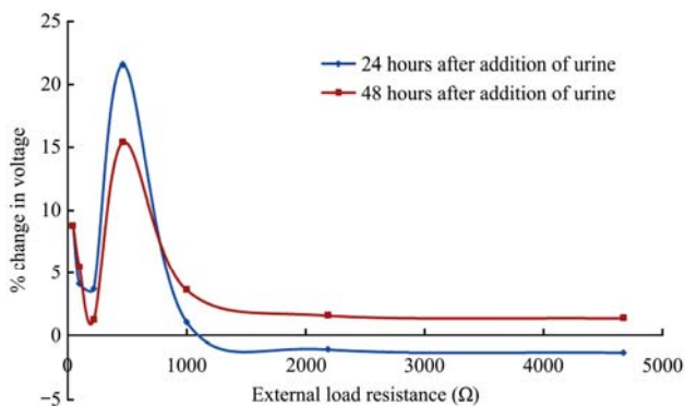
Figure 8 Percentage change in voltage across the external loads 24 hours and 48hours after urine addition to the MSCMFC
