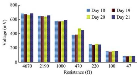
Figure 7 Voltage measured across external loads before (days 18 and 19) and after (days 20 and 21) urine addition
