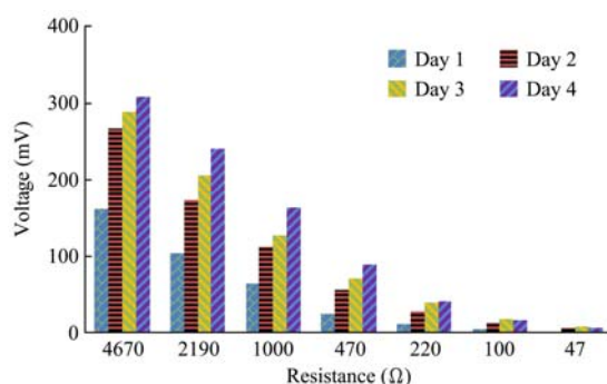
Figure 2 Voltage measured across external loads for the first four days (Days 1-4)
