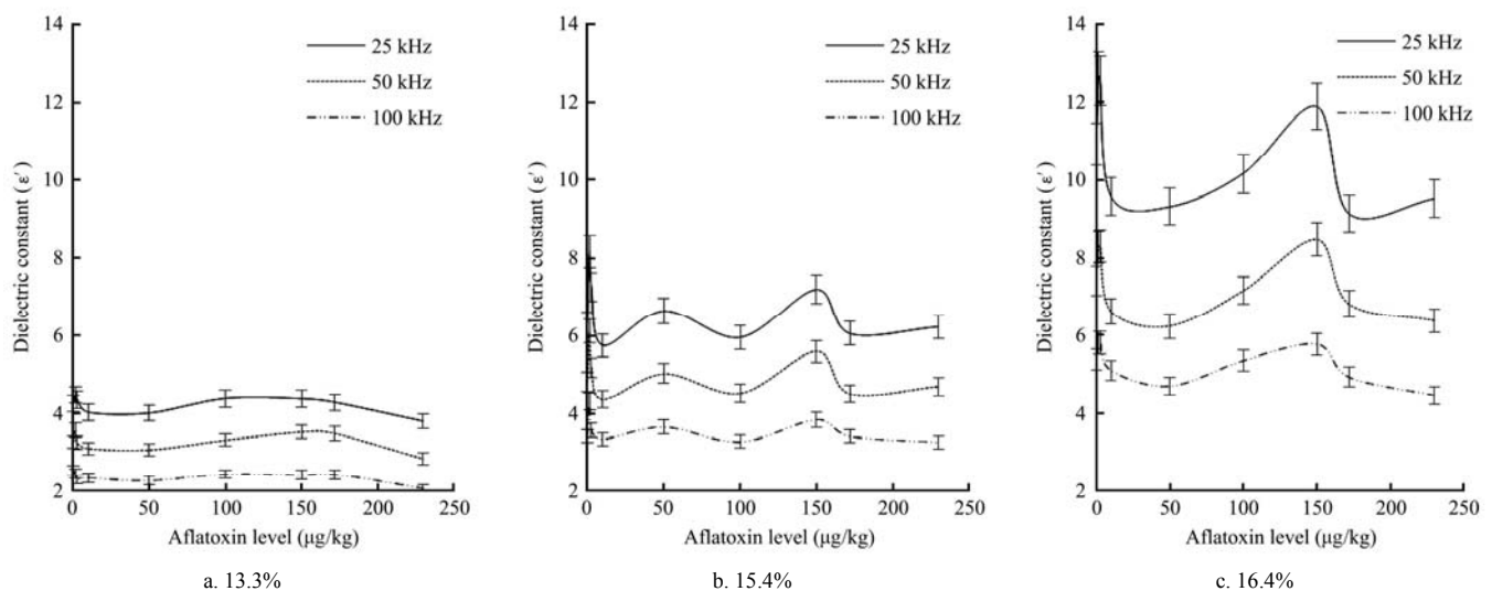
Figure 3 Variation of dielectric constant with aflatoxin contamination at specified frequencies for maize kernels at m.c. (w.b) ( \text{LSD}_{p<0.05} = 0.3154 , \text{CV} = 0.014 )
