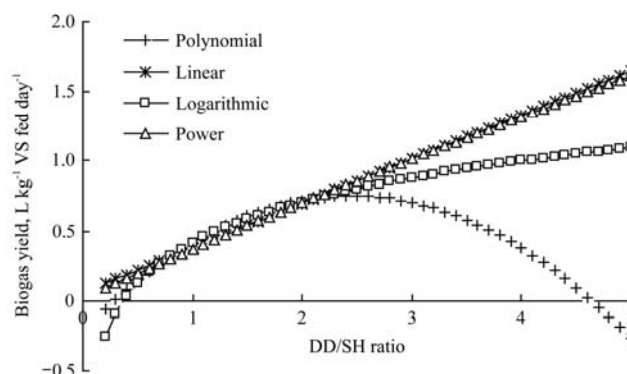
Figure 4 Regression curves relating DD/SH ratio and BY . Biogas production commenced at DD/SH ratio ≈ 0.3, peaked at ≈ 2.5 and ceased at ≈ 4.6
