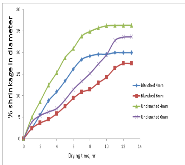
Figure 8 Effect of treatment, sample thickness and drying time on %shrinkage in diameter of cylindrical shaped sweet potato samples dried at 90°C
