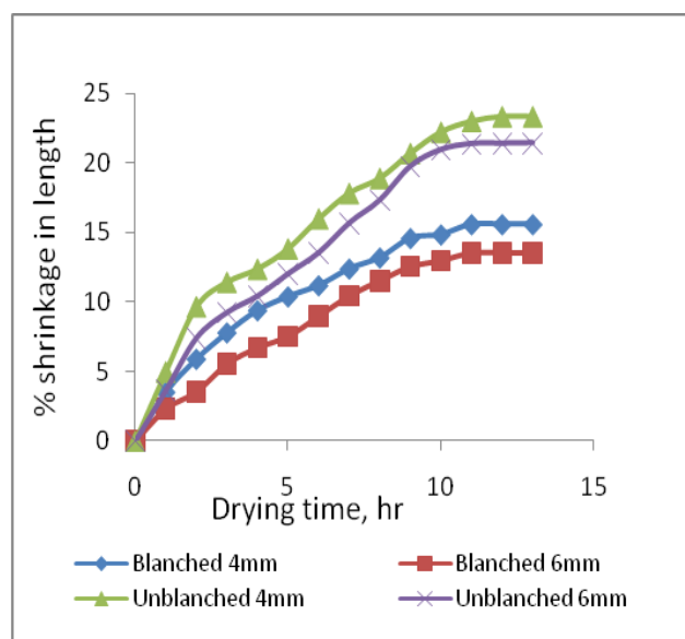
Figure 5 Effect of blanching, sample thickness and drying time on % shrinkage in length of rectangular shaped sweet potato samples dried at 90°C
