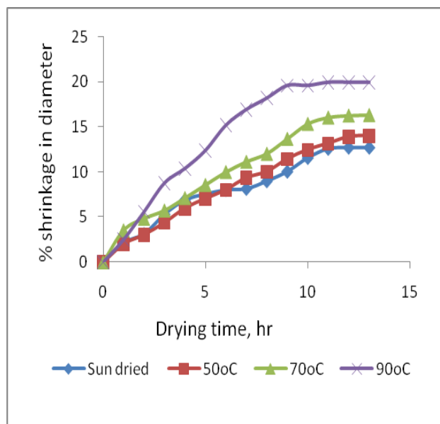
Figure 4 Effect of drying temperature and time on % shrinkage in diameter of blanching cylindrical shaped 6 mm thick sweet potato samples
