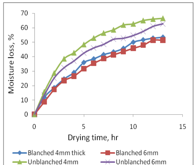
Figure 2 Effect of treatment, sample thickness and drying time on % moisture loss of rectangular shaped sweet potato slices oven dried at 90^{\circ}\text{C}
