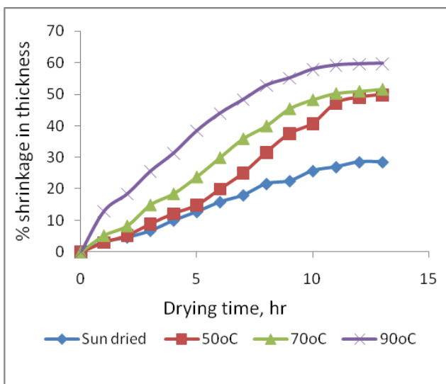
Figure 3 Effect of drying temperature and time on % shrinkage thickness in the blanching cylindrical shaped 4mm thick sweet potato samples
