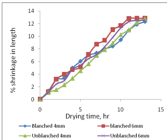
Figure 6 Effect of blanching, sample thickness and drying time on %shrinkage in length of rectangular shaped sweet potato samples dried at 50°C
