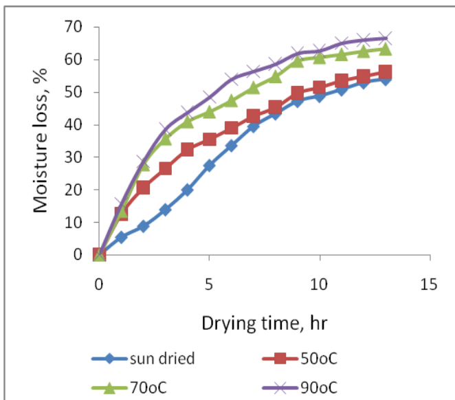
Figure 1 Effect of drying temperature and time on % moisture loss of un-blached rectangular shaped 4mm thick sweet potato samples
