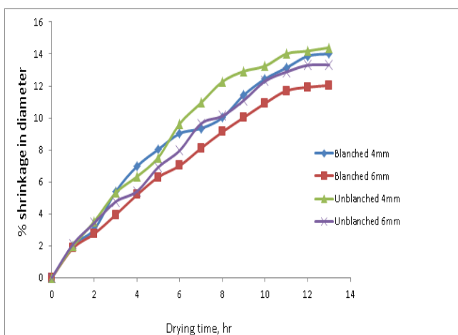
Figure 7 Effect of treatment, sample thickness and drying time on %shrinkage in diameter of cylindrical shaped sweet potato samples dried at 50°C
