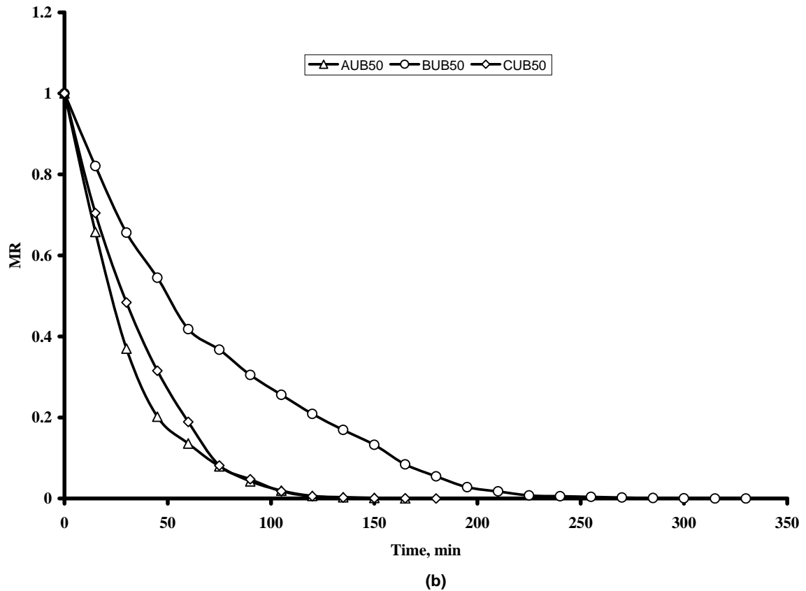
Figure 1 MR Variation with Time of (a) Blanched (b) Unblanched Potato Slices at 50°C
