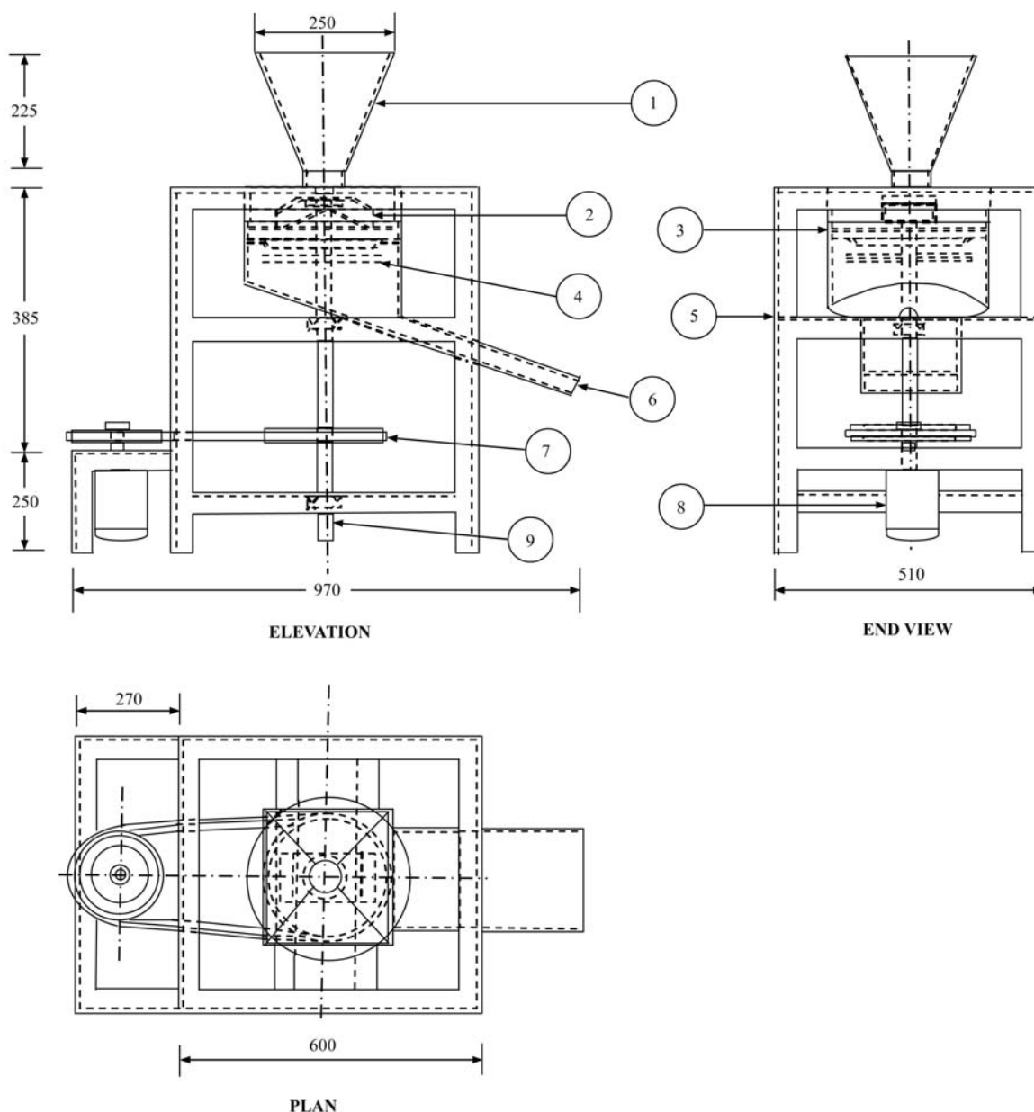
1. Feed hopper 2. Rotor 3. Shelling drum 4. Spinning disc 5. Frame 6. Delivery chute 7. Pulley 8. Electric motor 9. Shaft
