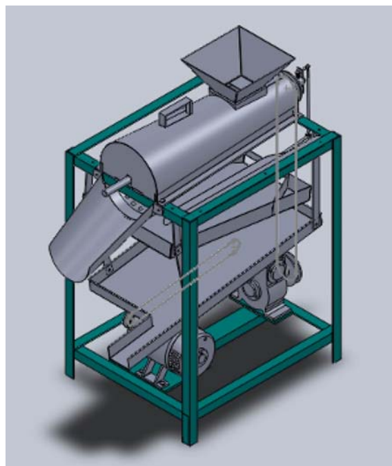
Figure 5 Isometric CAD view of pea depoding machine
