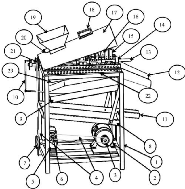
1. Frame 2. Motor 3. Motor pulley 4. Belts 5. Gear box 6. Gear driver pulley 7. Gear driven pulley 8. Second tray 9. First tray 10. Vibration assembly 11. Outlet pea grain guider 12. Trash guider 13. Main shaft 14. Bearing 15. L-shaped blades 16. Conveying blades 17. Upper cover 18. Handle 19. Hopper 20. Hopper plate 21. Main shaft pulley 22. Sieve 23. Side grain guider
