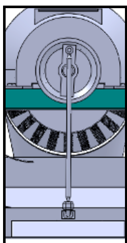
Figure 4 Vibrating assembly attached to pulley and first tray of the machine
