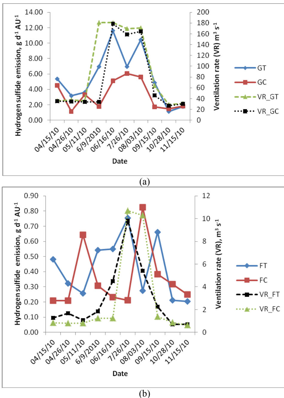
Figure 5. Variation of hydrogen sulfide emission a) between gestation treated (GT) and gestation untreated (GC) barn; and b) between farrowing treated (FT) and farrowing untreated (FC) barn. Ventilation rate (VR) in the barns are shown on the secondary axis..
