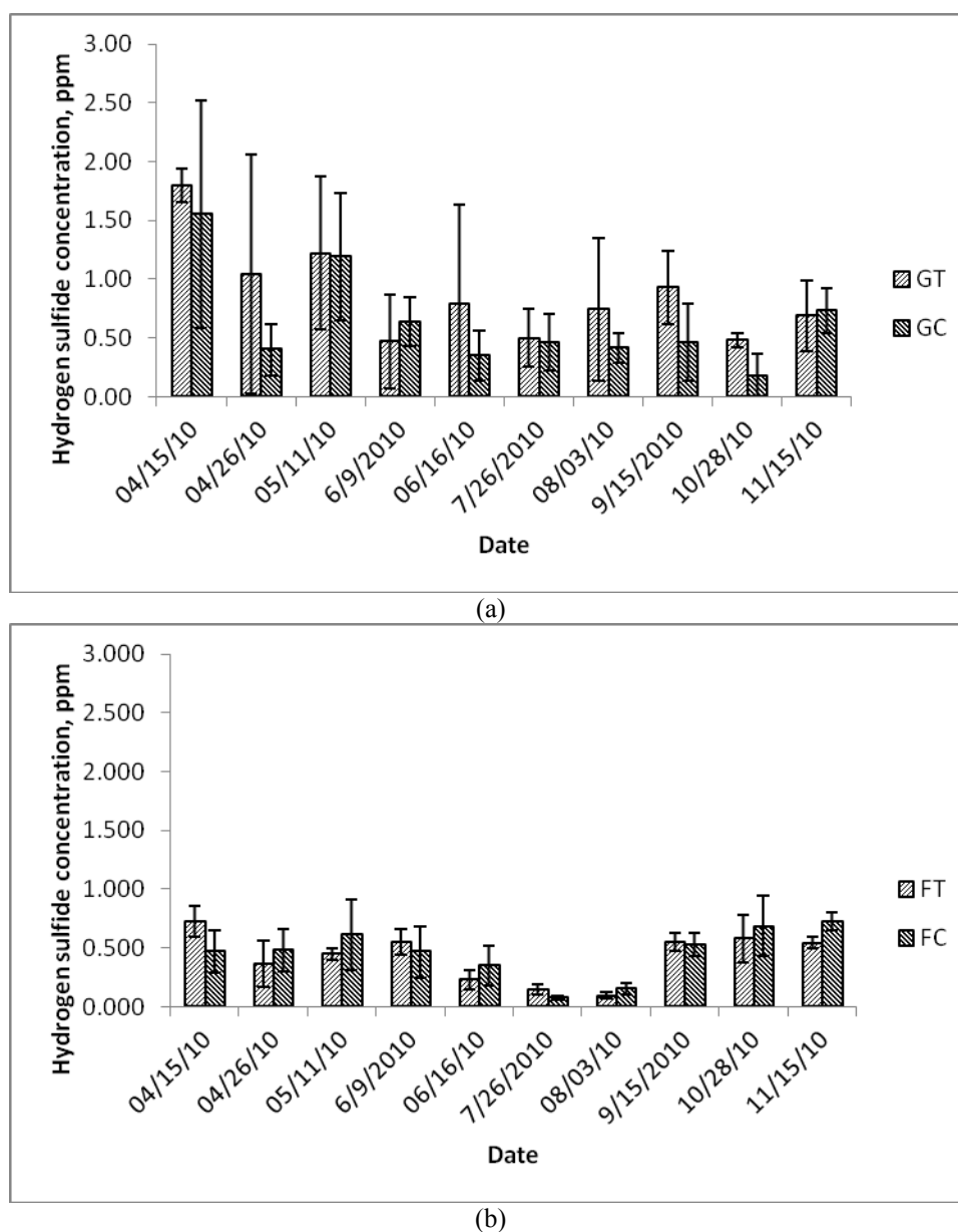
Figure 4. Variation of hydrogen sulfide concentration a) between gestation treated (GT) and gestation untreated (GC) barn; and b) between farrowing treated (FT) and farrowing untreated (FC) barn. Error bars represent standard deviation.
