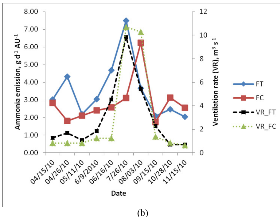
(b) Figure 3. Variation of ammonia emission: a) between gestation treated (GT) and gestation untreated (GC) barn; and b) between farrowing treated (FT) and farrowing untreated (FC) barn. Ventilation rate (VR) in the barns are shown on the secondary axis.
