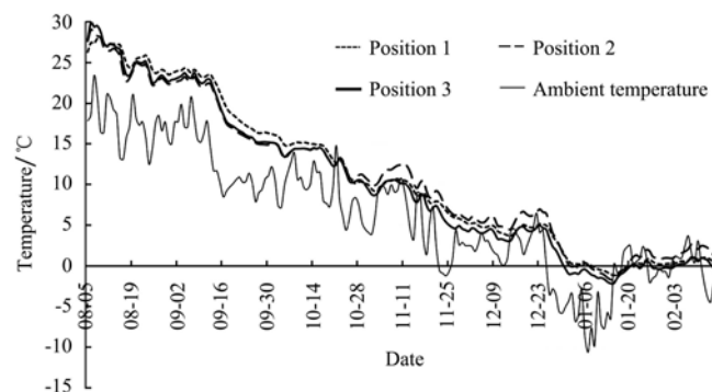
Figure 2 Temperature data in the polyethylene bag no. 2 during the storage in comparison with the ambient temperature
