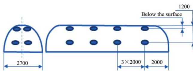
Figure 1 Schematic illustration of the polyethylene bag with the measurement points
