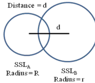
Figure 1 Overlap of two SSLs.
