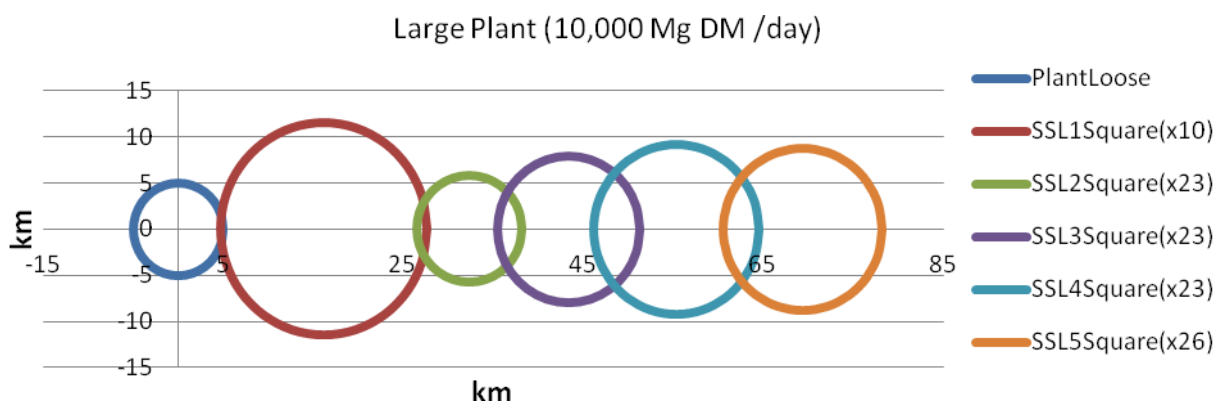
Figure 6 Large plant handling locations.
