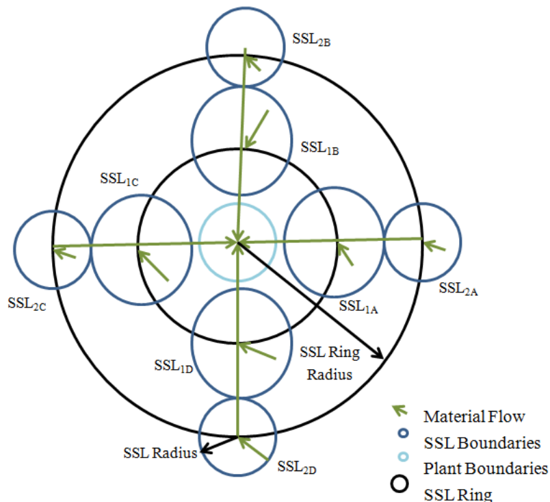
Figure 2 Satellite storage locations.
