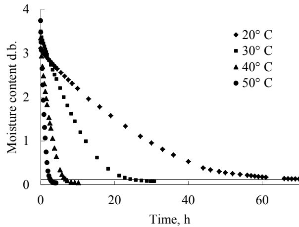
Figure 2. Moisture content versus time at different temperatures
