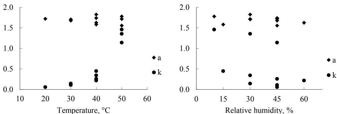
Figure 4. Plots of the Two-term exponential model parameters versus temperature (left) and relative humidity (right)
