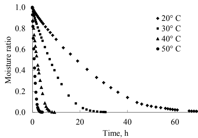
Figure 1. Moisture ratio versus time at different temperatures
