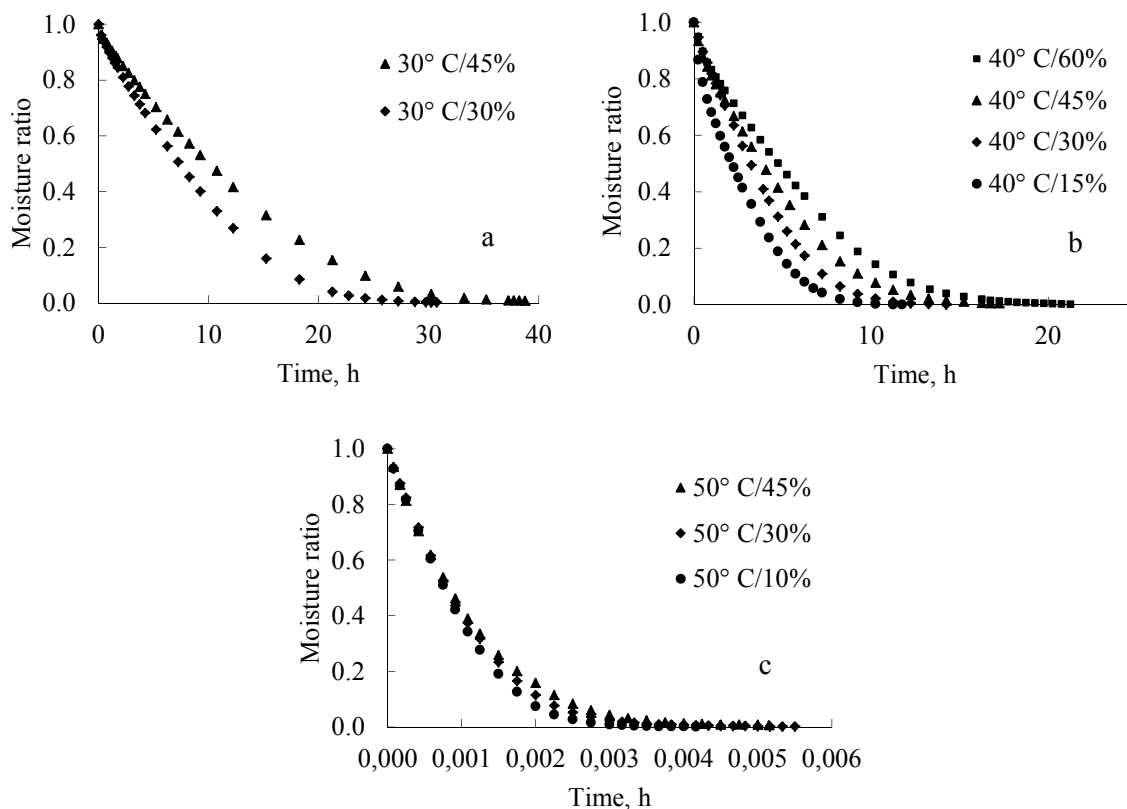
Figure 3. Effect of air relative humidity on drying curves at 30° C (a), 40° C (b), and 50° C (c)
