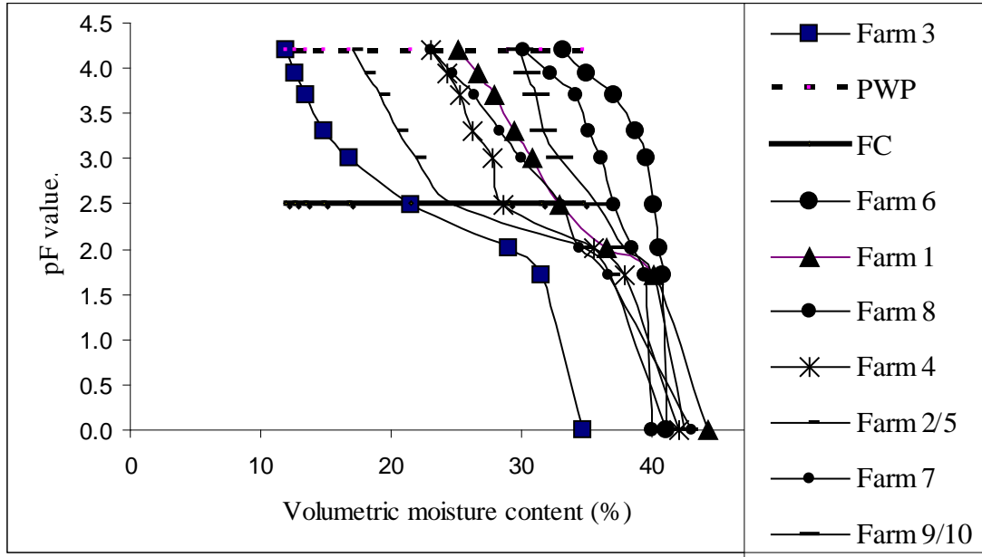
Figure 5 Pf values versus volumetric moisture content
