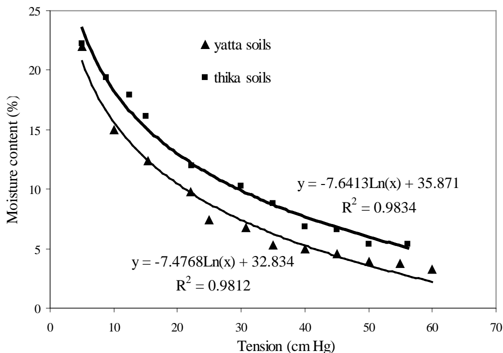
Figure 4 Calibration curve for the tensiometers
