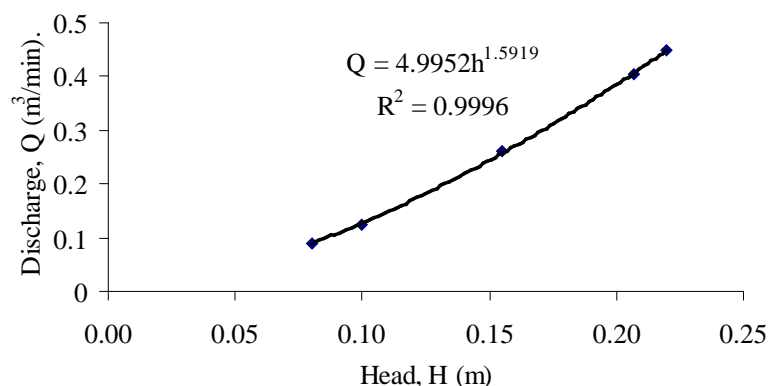
Figure 3 Calibration curve of the Parshall flume
