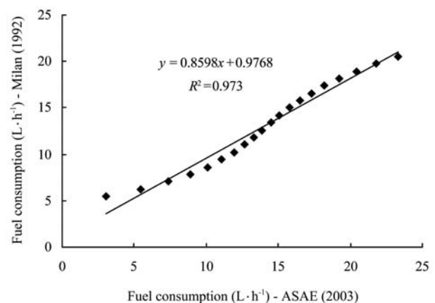
Figure 3 Relation between distinct models for fuel consumption
