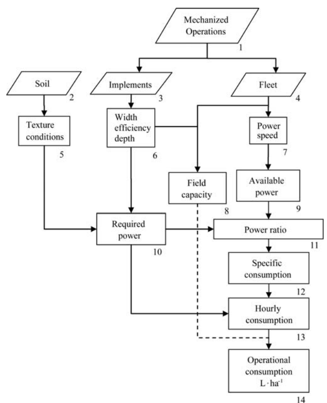
Figure 2 Data flow for fuel consumption
