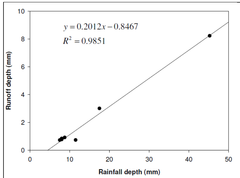
Figure 5. Rainfall- runoff relation
