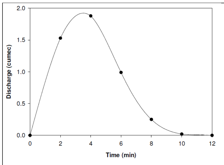
Figure 6. Representative Unit hydrograph
