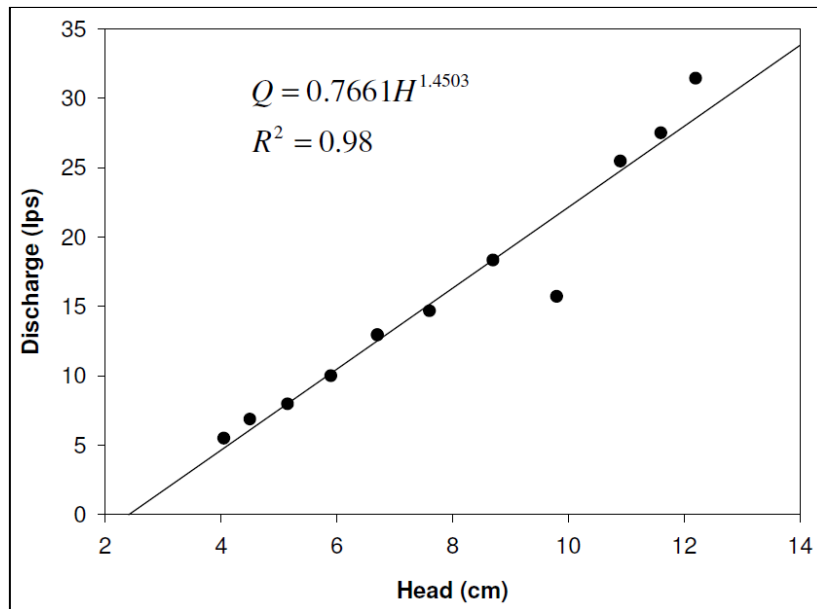
Figure 4. Head – discharge relationship
