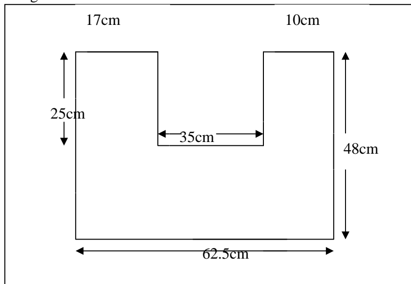
Figure 2. Dimensions of rectangular notch
