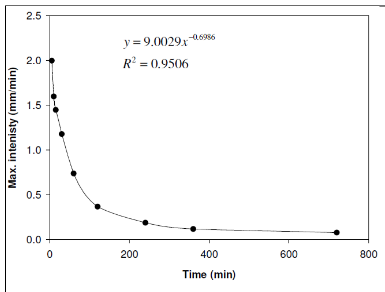
Figure 7. Maximum Intensity –Duration relationship
