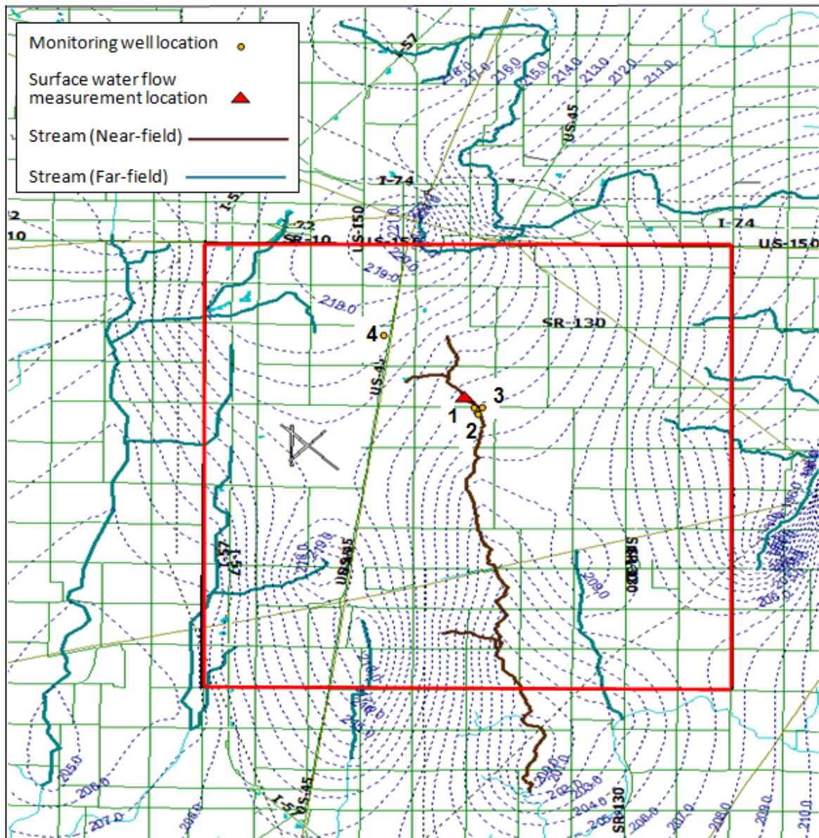
Figure 2 GFLOW calibration of hydraulic conductivity for the Upper Embarras River site
