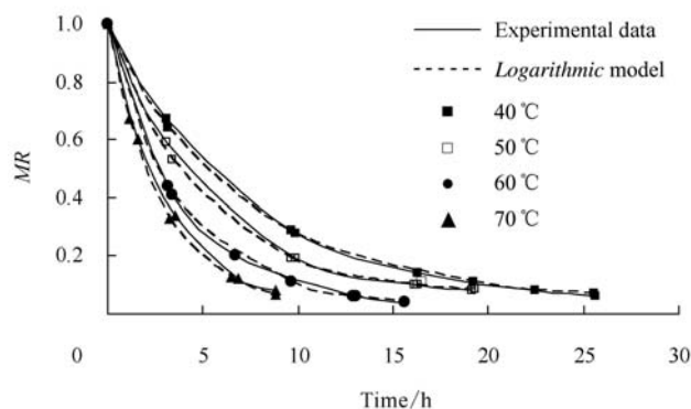
Figure 2 Experimental and predicted moisture ratio by the Logarithmic model versus drying time for air velocity of 1 m/s
