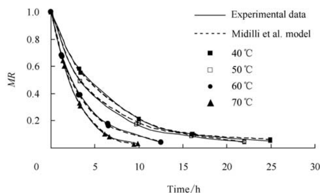
Figure 3 Experimental and predicted moisture ratio by the Midilli et al. model versus drying time for air velocity of 2 m/s
