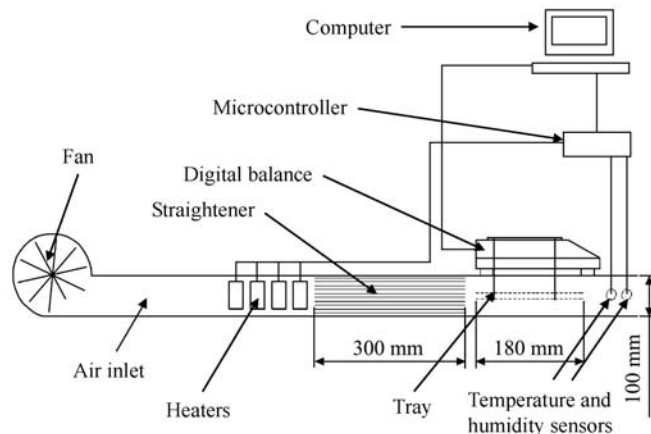
Figure1 Schematic of thin-layer drying equipment
