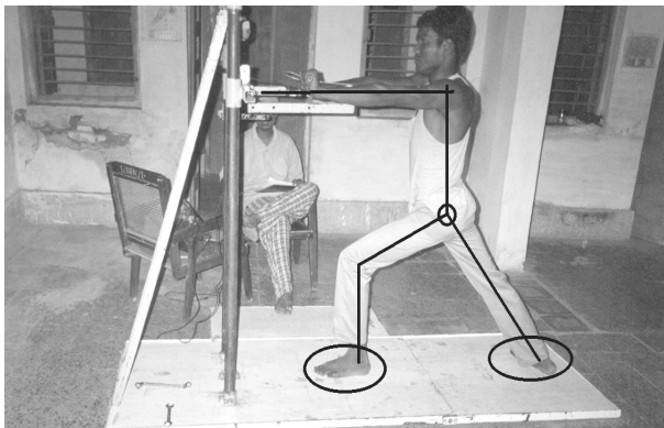
Figure 1 Measurement of push force with both hands in standing posture in horizontal plane
