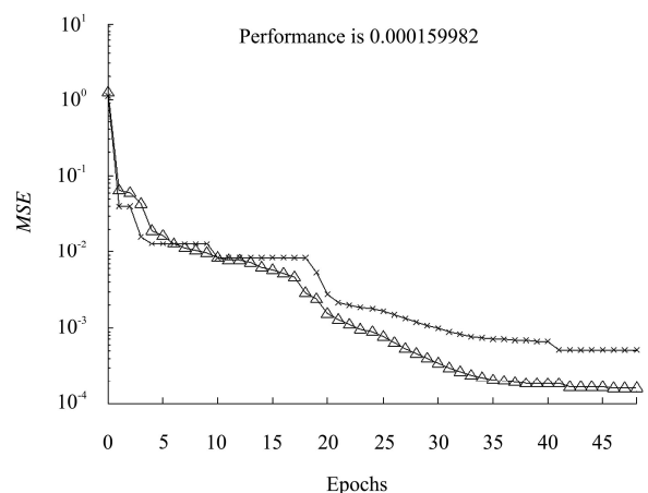
Figure 5 Mean square error of training and testing patterns for the best ANN
