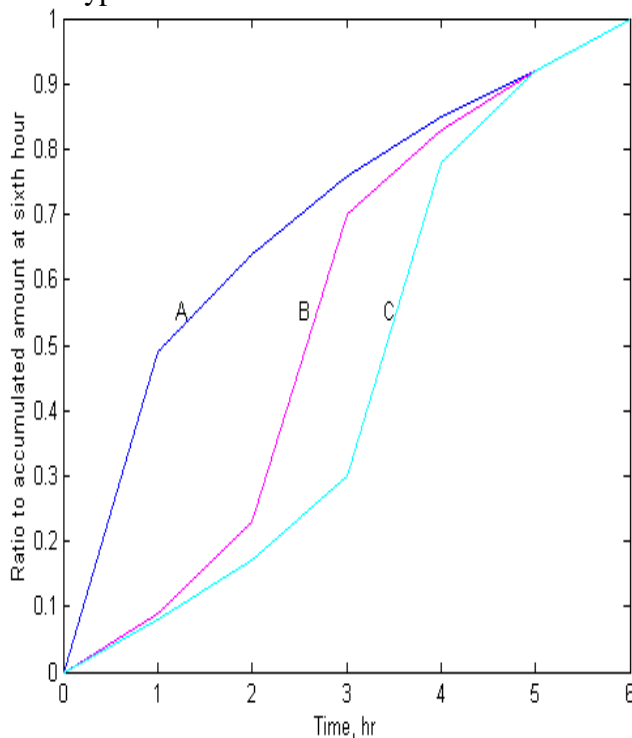
Figure 4: Generalized accumulated rainfall curves for A (advanced), B (intermediate), and C (retarded) types of storms. (USDA SCS, 1955)
