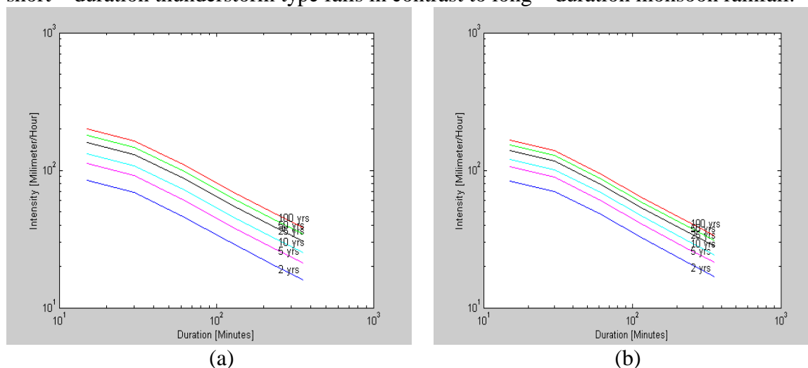
Figures 6: Intensity-Duration-Frequency Curves for Onitsha obtained by (a) Graphical Method (b) Statistical Method
