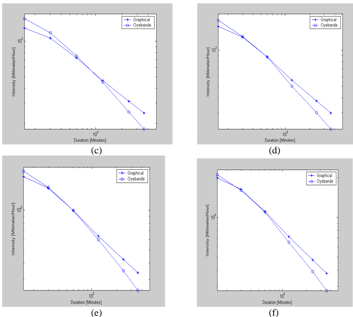
Figure 8: IDF Curves obtained by the Graphical Method and Oyebande (1983) for Enugu location (a) 2-year Return Period. (b) 5-year Return Period. (c) 10-year Return Period. (d) 25-year Return Period. (e) 50-year Return Period. (f) 100-year Return Period
