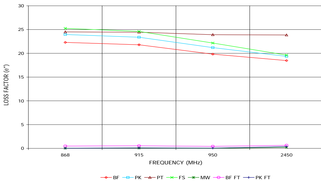
Figure 3 Mean dielectric loss factors of all test samples at 7 °C as functions of RFID relevant frequencies.
