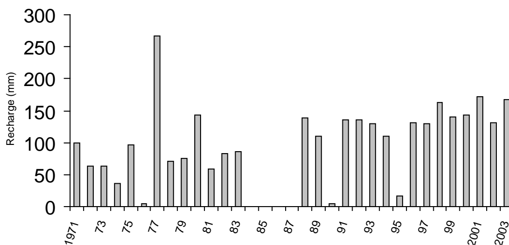
Figure 5 : Recharge trend between Wudil and Hadejia
