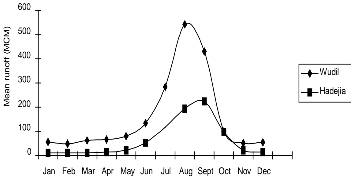
Figure 3: Hydrograph of the Hadejia River at Wudil and Hadejia
