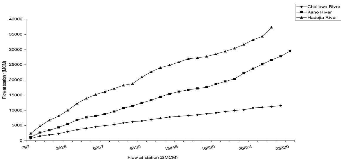
Figure 2: Double mass curve of major rivers in the study area
