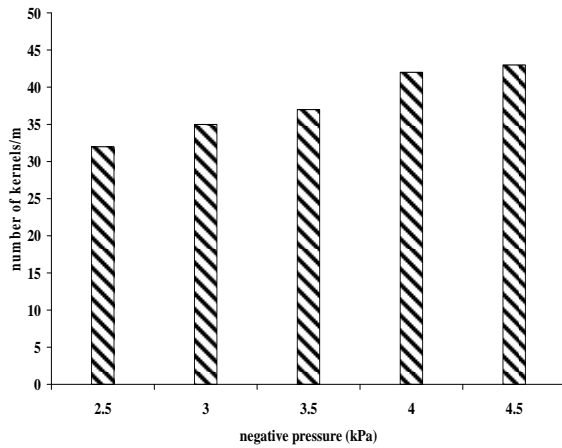
Figure 9 Effect of negative pressure on number of kernels per meter
