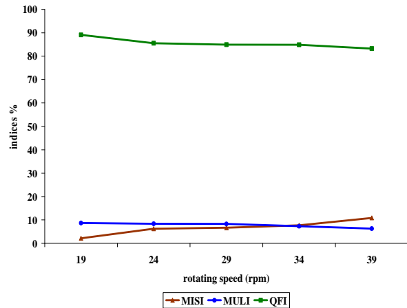
Figure 8 Effect of rotating speed on performance indices
