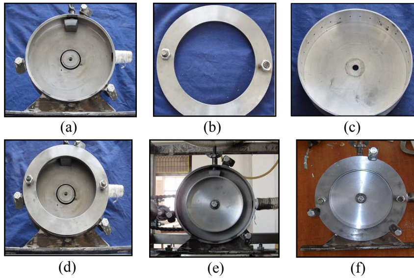
Figure 3: Main parts of the pneumatic precision metering device for wheat (a) the main shield with air cut-off device (b) the removable ring (c) the seed plate (d) the ring fixed to the main shield (e) the seed plate inside the main shield (f) the main shield seed plate and removable ring fixed together as one unit
