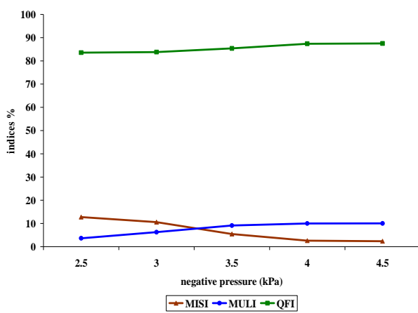
Figure 7 Effect of negative pressure on performance indices
