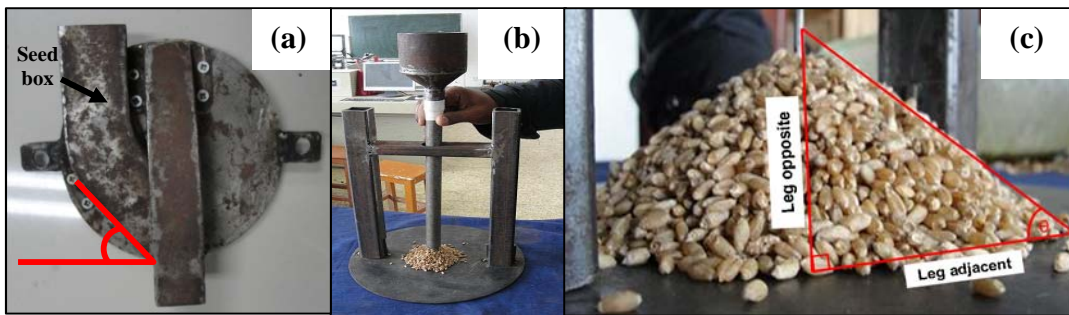
Figure 1 Determination of angle of repose (a) the angle of seed box (b) apparatus used in the test (c) measurement of opposite and adjacent legs
