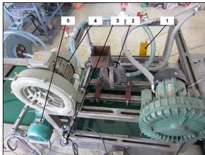
Figure 5 Metering device on the test stand
