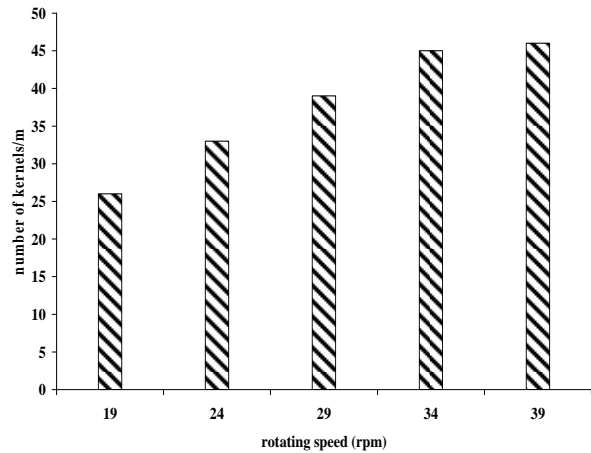
Figure 10 Effect of rotating speed on number of kernels per meter
