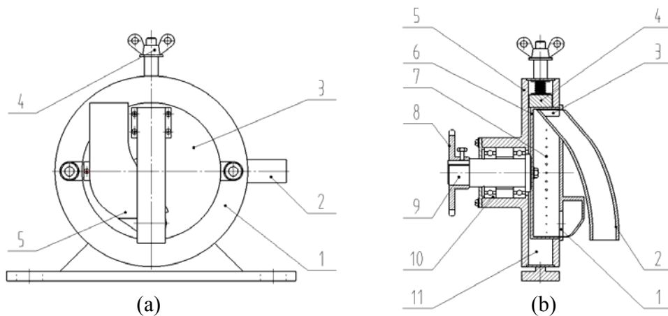
Figure 2 Schematic diagram of the pneumatic precision metering device for wheat
