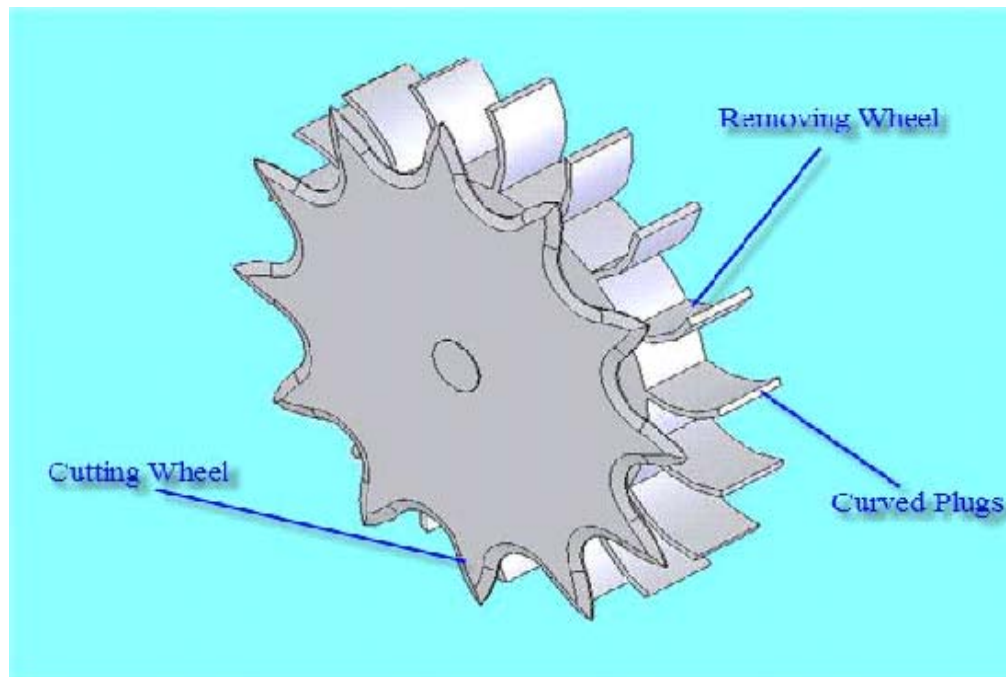
Figure 2. Geometry of the powered residue management device.
