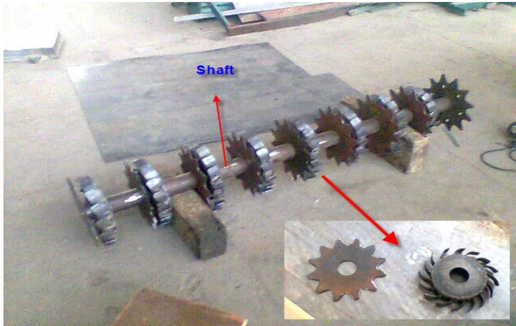
Figure 3. Arrangement of the residue manager parts on its shaft.
