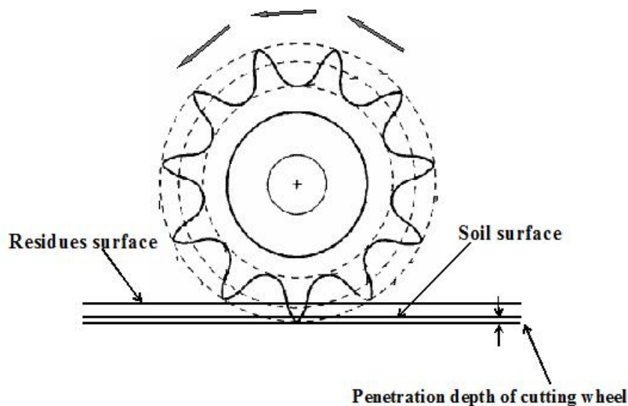
Figure 1. Cutting wheel related to soil and residue surfaces.
